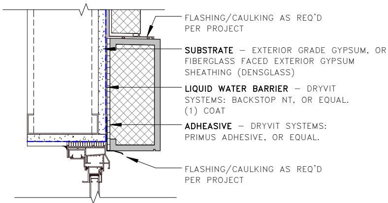
EXTERIOR GYPSUM SHEATHING
