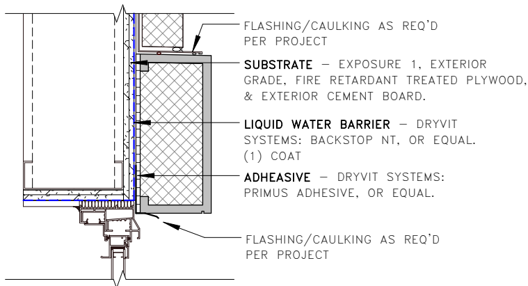
EXTERIOR WOOD SHEATHING
