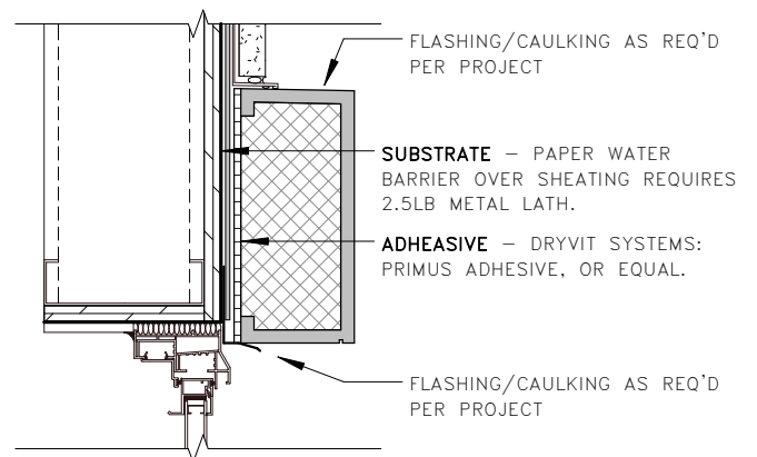
PAPER WATER BARRIER
