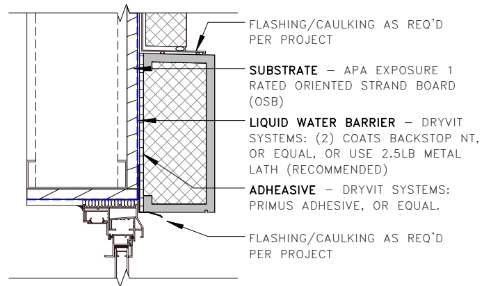
EXTERIOR PARTICAL BOARD (OSB)
