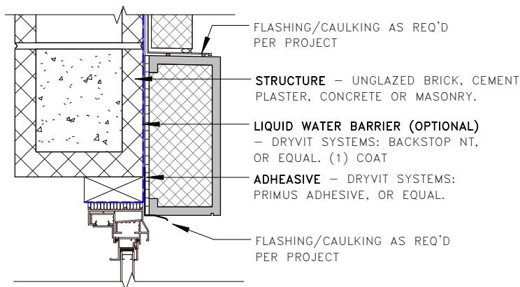
CONCRETE & MASONRY
