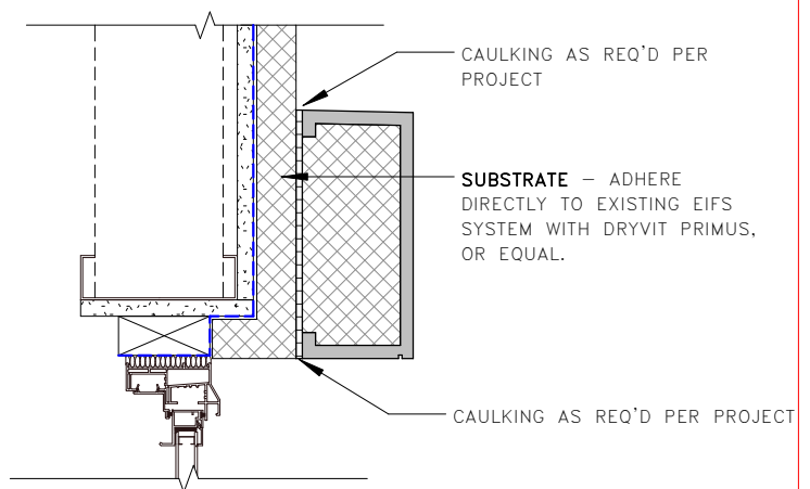
EXISTING EIFS
